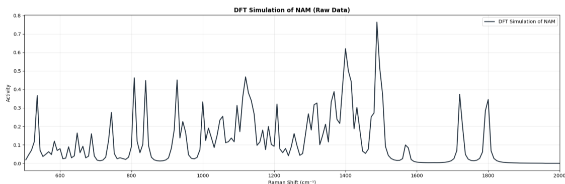
Figure 4.3: Simulated Raman spectrum of N-Acetylmuramic Acid generated using DFT calculations.
