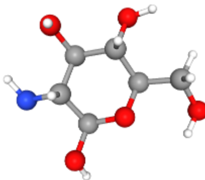
D-Glucosamine
