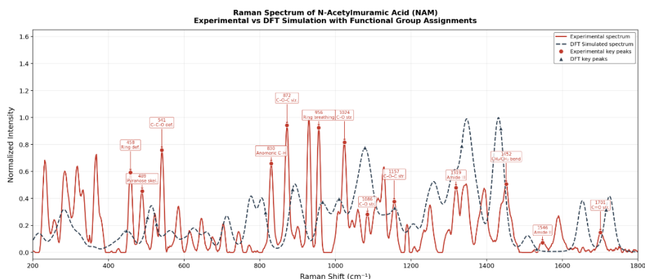
Figure 4.8: Comparative overlay of experimental and simulated Raman spectra of N-Acetylmuramic Acid.
