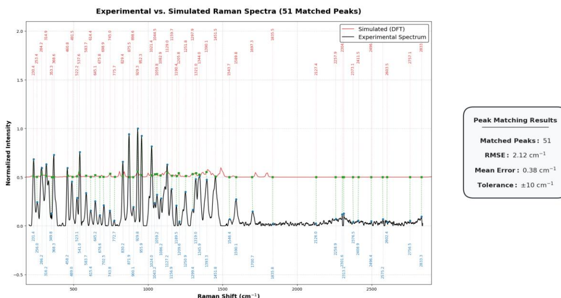
Figure 4.9: Peak matching and error analysis between experimental and simulated NAM spectra.
