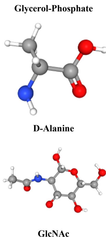
Figure 4.10: Representative fragment models used for theoretical simulation of Lipoteichoic Acid (LTA).
