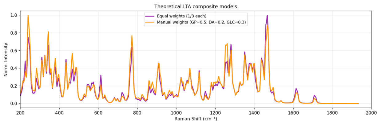
Figure 4.12: Composite theoretical Raman spectrum of Lipoteichoic Acid generated from weighted combination of simulated fragments.
