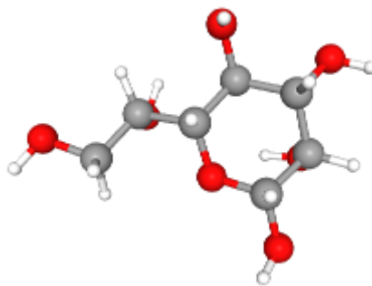
L-glycero-D-manno-heptose
