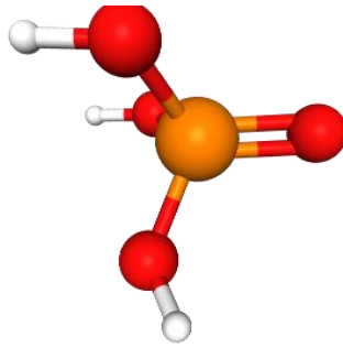
Phosphoric Acid
