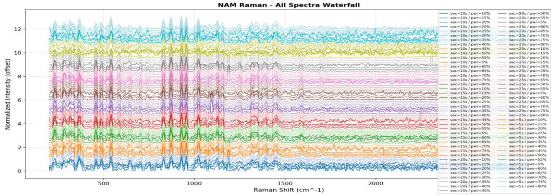
Figure 4.4: Stacked Raman spectra of NAM recorded under multiple laser power and integration time conditions.
