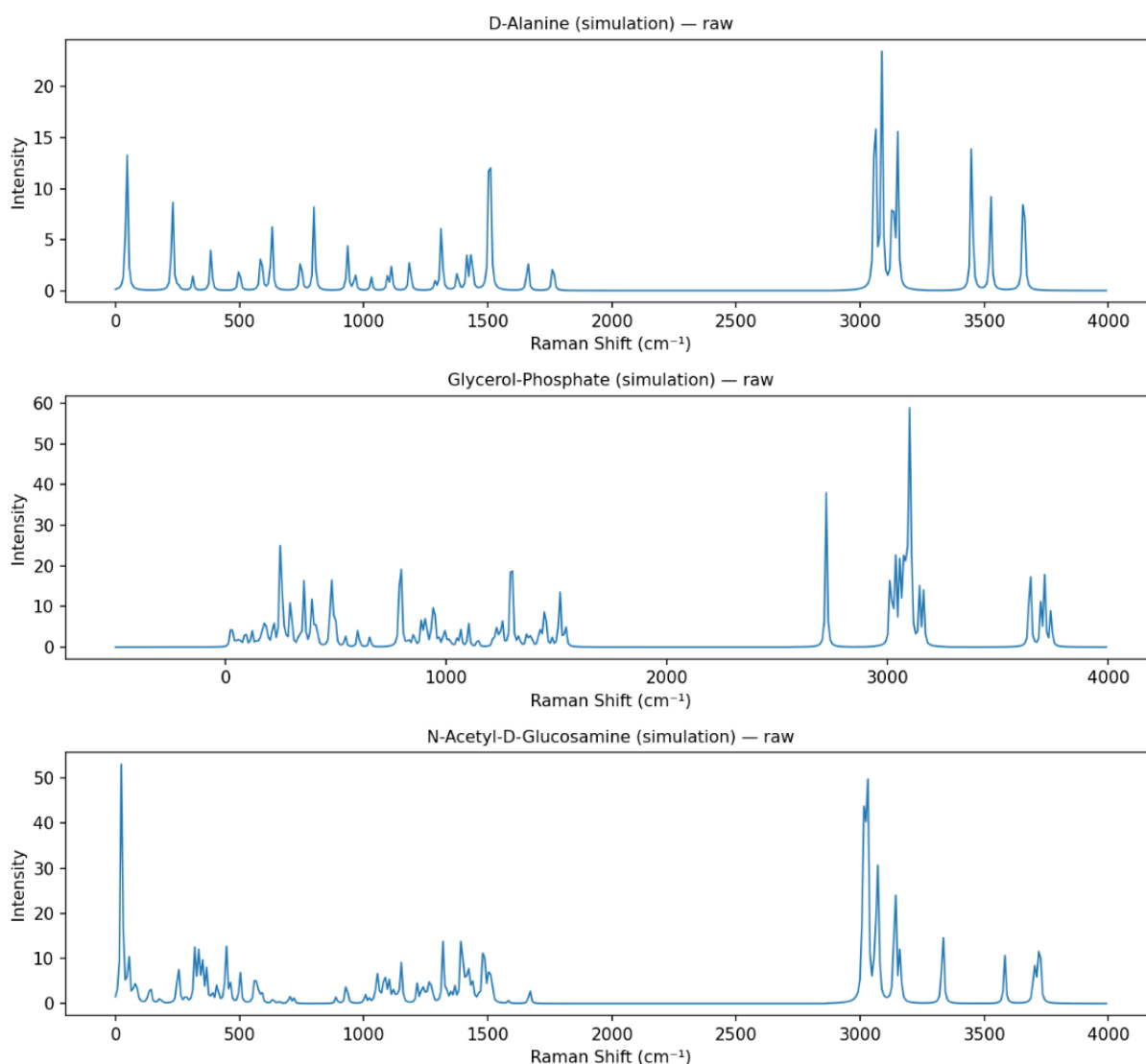
Figure 4.11: Simulated Raman spectra of individual LTA fragments: Glycerol-Phosphate, D-Alanine, and GlcNAc.
